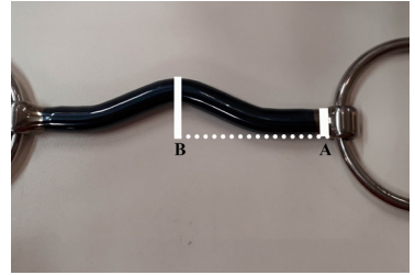
Ported bit. The max. height of the port (B) shall be 2 \times A .
